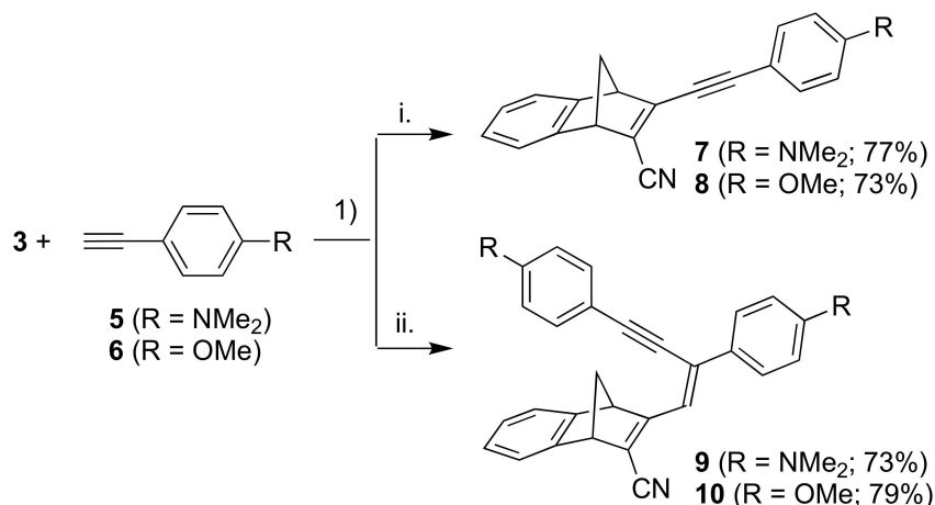
Scheme 3. Reagents and conditions: (1) Pd(PPh 3 ) 2 Cl 2 , CuI, THF/Et 3 N; i. alkyne: 1 equiv.; ii. alkyne: excess.
